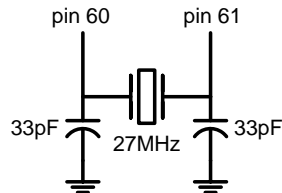
Figure 7. Crystal and Load Circuit
