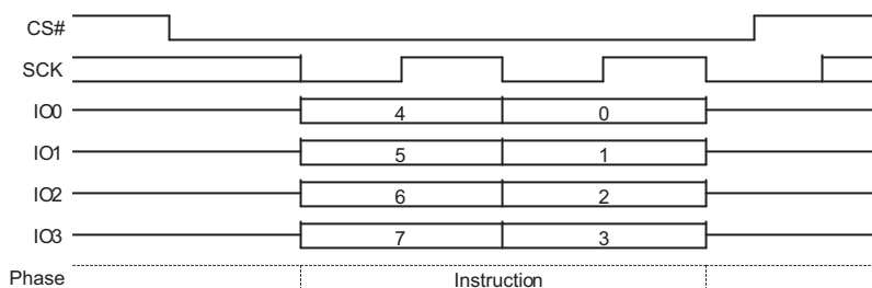
Figure 10.79 RES Command Sequence QPI Mode
