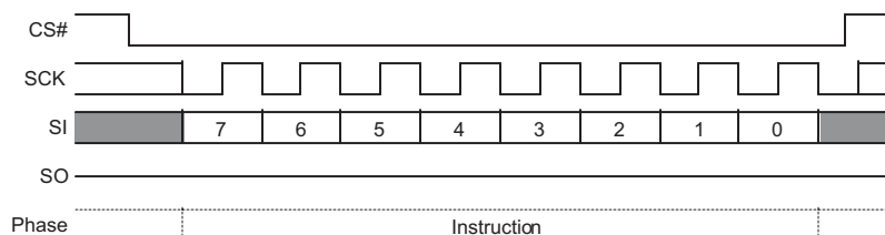
Figure 10.78 Release from Deep Power-Down Command Sequence
