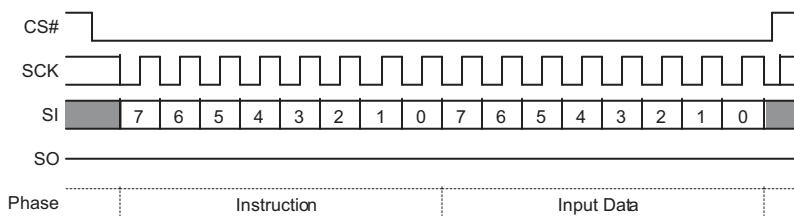
Figure 10.20 Write VDLR (WVDLR) Command Sequence
