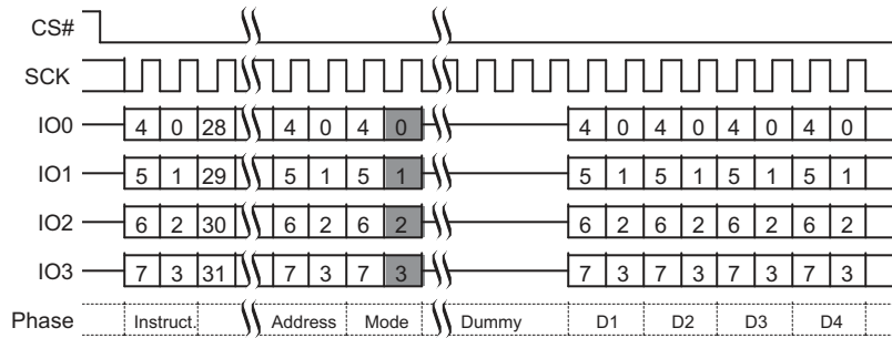
Figure 4.11 DDR Quad I/O Read
