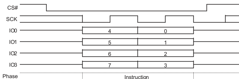
Figure 10.77 DPD Command Sequence QPI Mode
