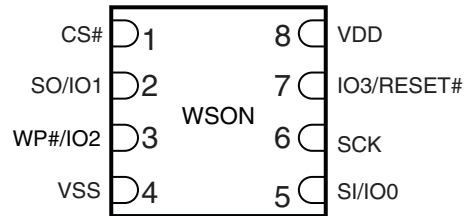
Figure 7.3 8-Connector Package (WSO N 6x8), Top View
