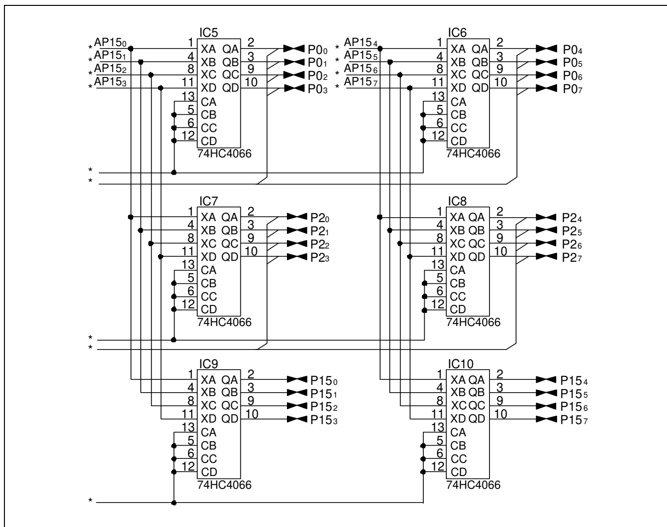
Figure 4.3 Connection diagram (3/3)
