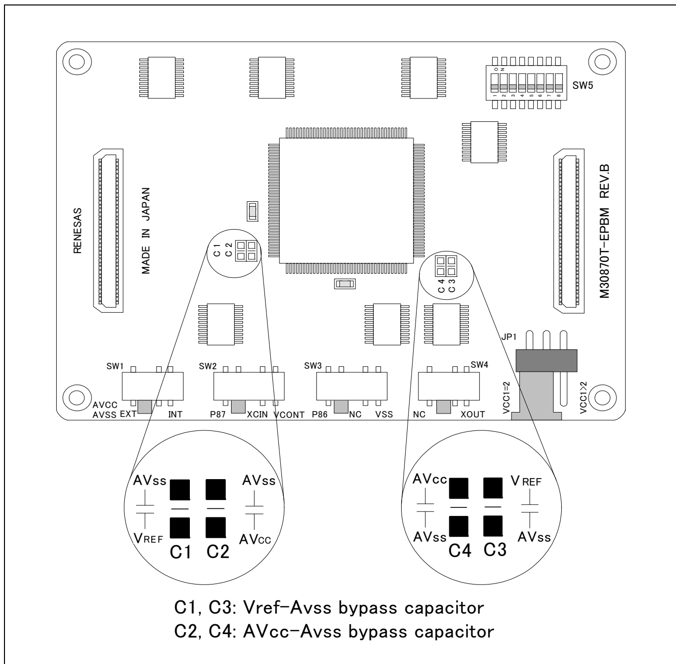
Figure 2.24 Foot pattern for the A/D conversion bypass capacitor on the M30870T-EPBM REV.B
