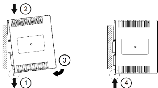
Fig. 2.1 Mounting
