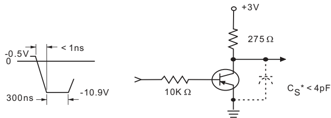
Delay and Rise Time Equivalent Test Circuit
