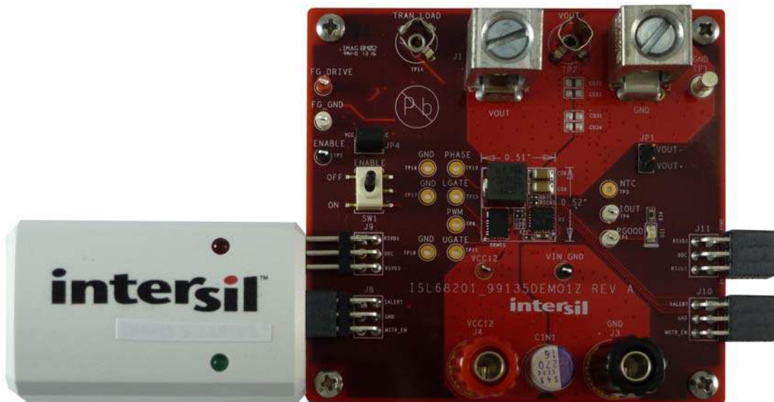
FIGURE 5. ISL68201-99135DEMO1Z DEMONSTRATION KIT SETUP
