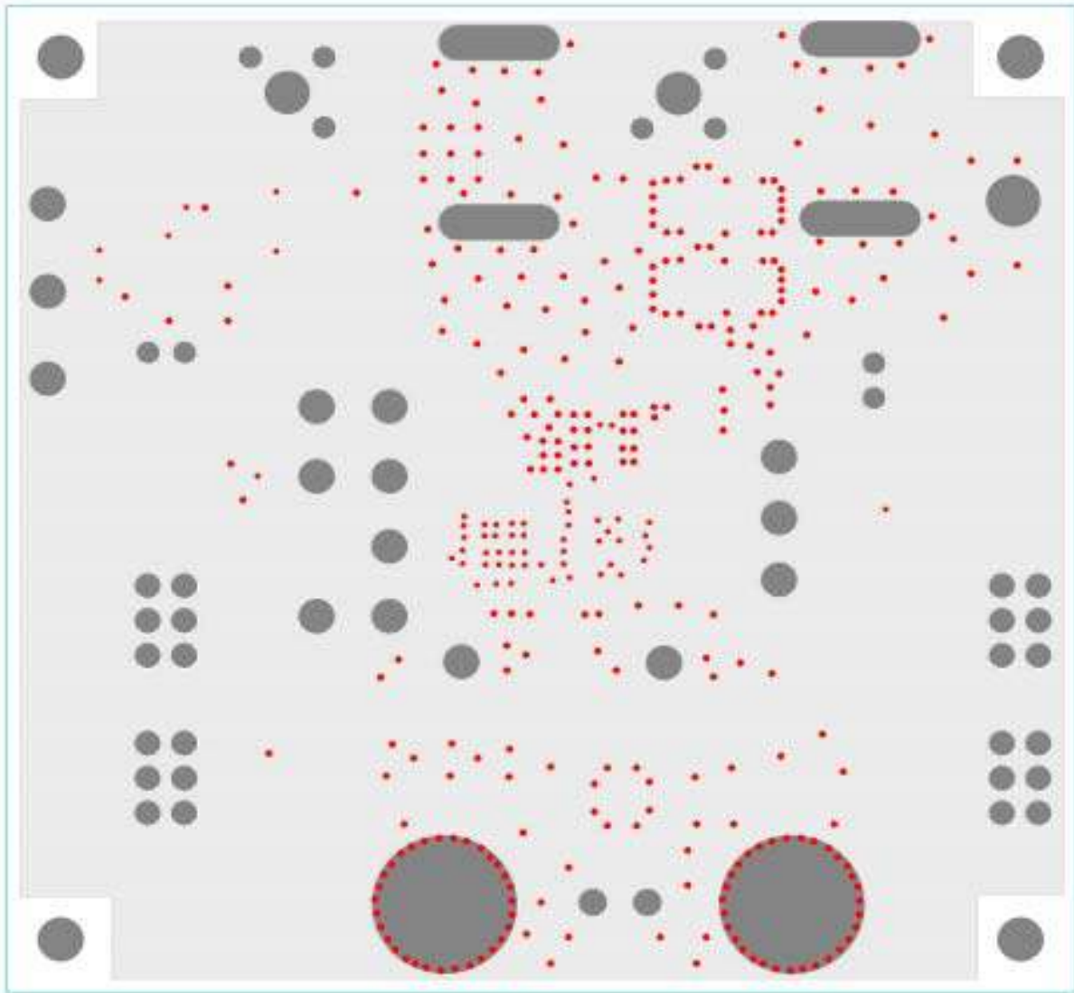
FIGURE 37. PCB - INNER LAYER 2 (TOP VIEW)
