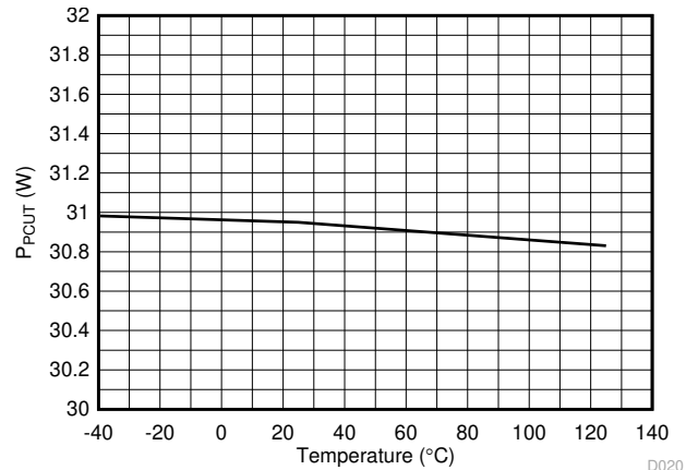
Figure 7-20. 2-Pair PCut Threshold (30W) vs Temperature
