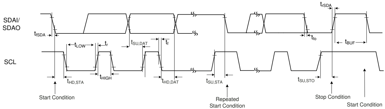
Figure 8-1. I 2 C Timings
