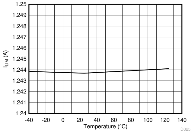
Figure 7-25. 2x Mode (2xFBn = 1) Current Limit vs Temperature
