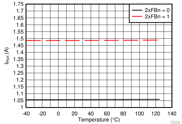
Figure 7-26. I SHORT Threshold vs Temperature
