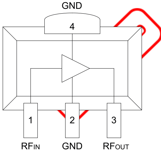
Figure 2: Pin Out
