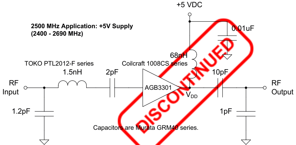
Figure 32: 2500 MHz Application Circuit (50Ω Terminations)
