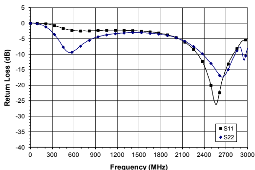
Figure 31: Return Loss vs. Frequency (V SUPPLY = +9 VDC, 2500 MHz Application Circuit)
