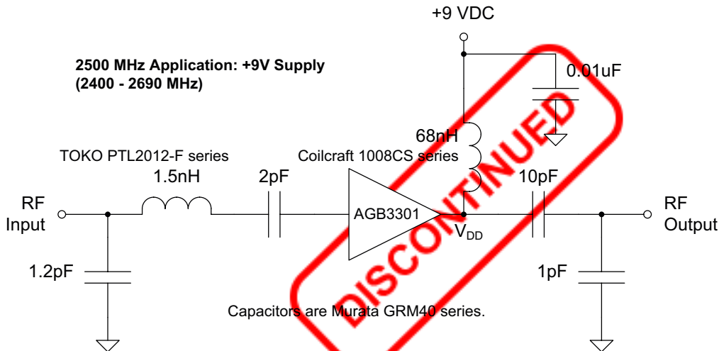
Figure 28: 2500 MHz Application Circuit (50Ω Terminations)
