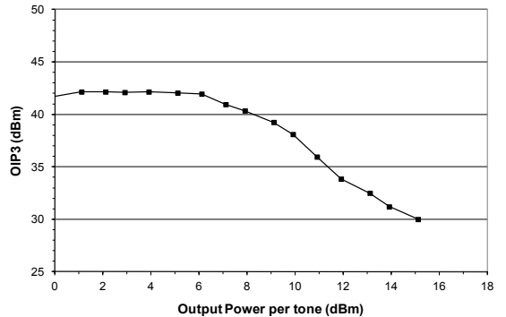
Figure 33: Output 3rd-Order Intercept vs. Power (V SUPPLY = +5 VDC, 2500 MHz Application Circuit)
