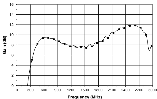
Figure 30: Gain vs. Frequency (V SUPPLY = +9 VDC, 2500 MHz Application Circuit)
