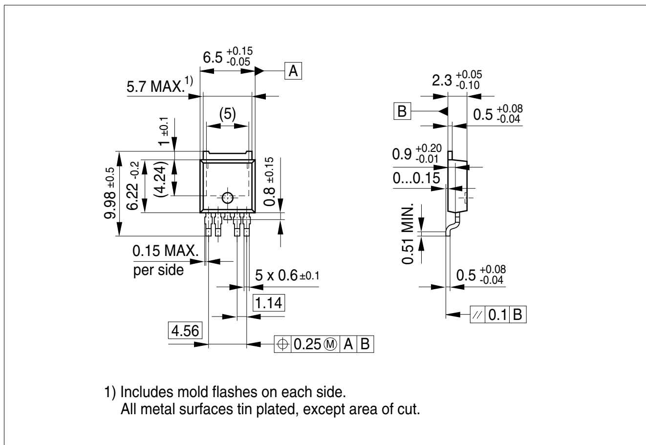
Figure 7 PG-T0252-5 1)
