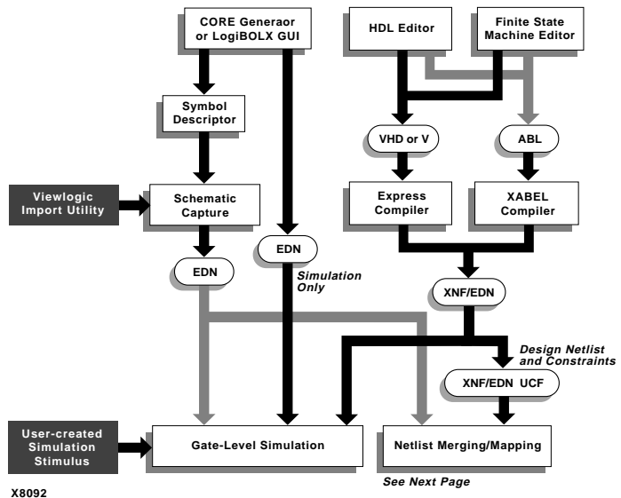
Figure D-1 Manipulation of Netlist and Constraint Files for FPGAs (Part 1)
