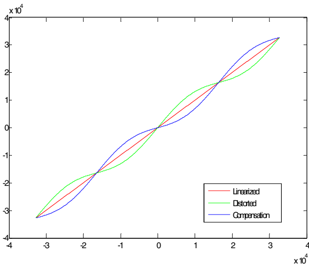
Fig. 3–4: Linearization - Principle
