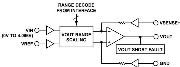
Figure 53. Voltage Output
