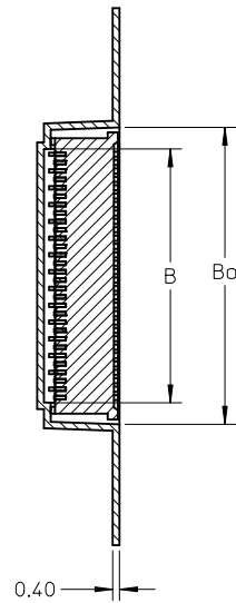
SECTION Y-Y
