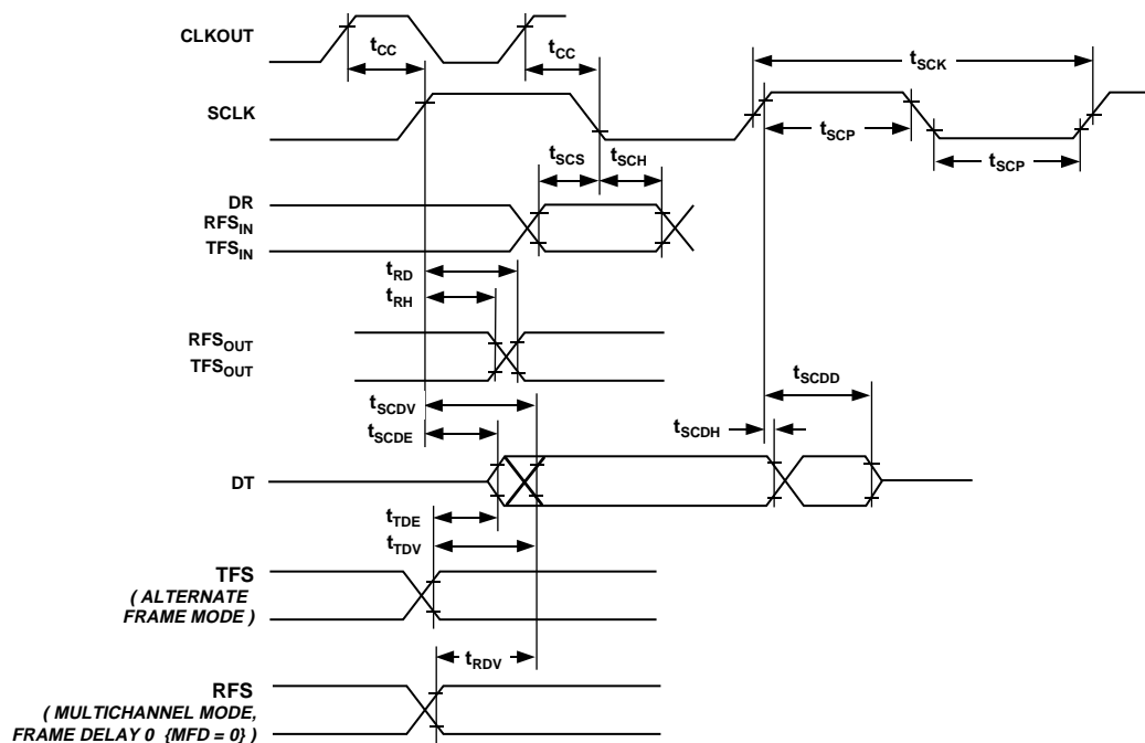
Figure 44. Serial Ports
