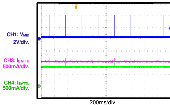
LS Cell Balance I_{CC} = 1A , I_{SYS} = 0A , HS cell is 3.6V and LS cell is 3.8V , balance enabled, balance resistor is 17m\Omega
