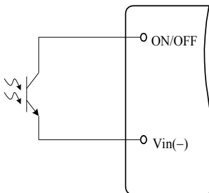
Figure 10. Opto Coupler Enable Circuit
