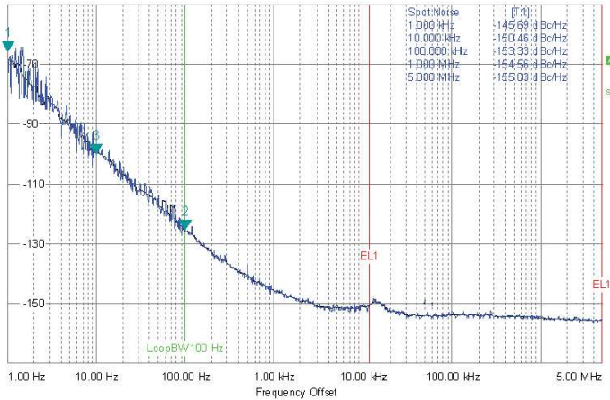
Typical Phase Noise for DOCSC012F-024.57M
