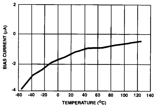
FIGURE 30. +INPUT BIAS CURRENT vs TEMPERATURE
