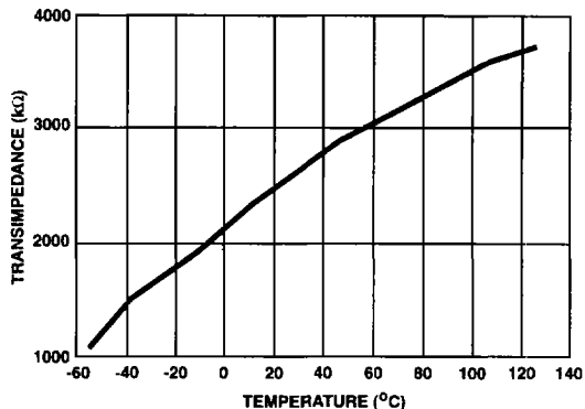
FIGURE 32. TRANSIMPEDANCE vs TEMPERATURE
