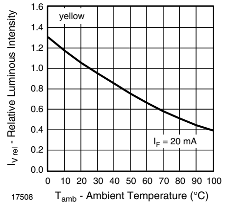
Fig. 16 - Relative Luminous Intensity vs. Ambient Temperature
