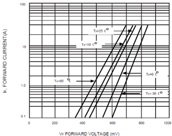
FIG. 2-TYPICAL FORWARD CHARACTERISTICS
