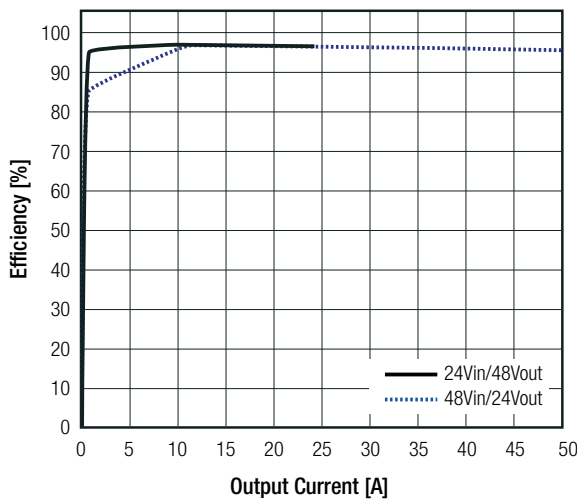
Efficiency vs. Load
