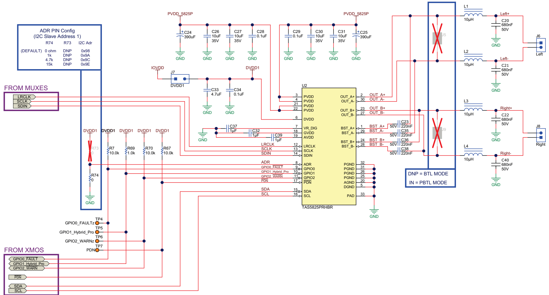
Figure 4. TAS5825PEVM Schematic (3 of 4)
