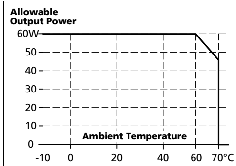
Fig. 14-1 Output power vs. ambient temp.
