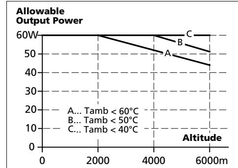
Fig. 14-2 Output power vs. altitude
