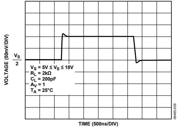
Figure 9. Small Signal Transient Response
