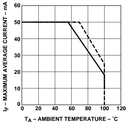
Figure 1. Maximum forward current vs. ambient temperature. Derating based on T_{JM\text{MAX}} = 130^{\circ}\text{C} .
