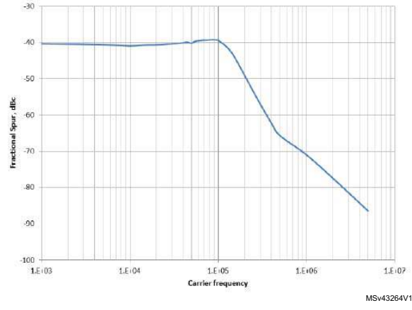
Figure 16. 10 kHz and 2.5 MHz fractional spur (integer boundary, 5.0 V supply, F_{PFD}=50 MHz)
