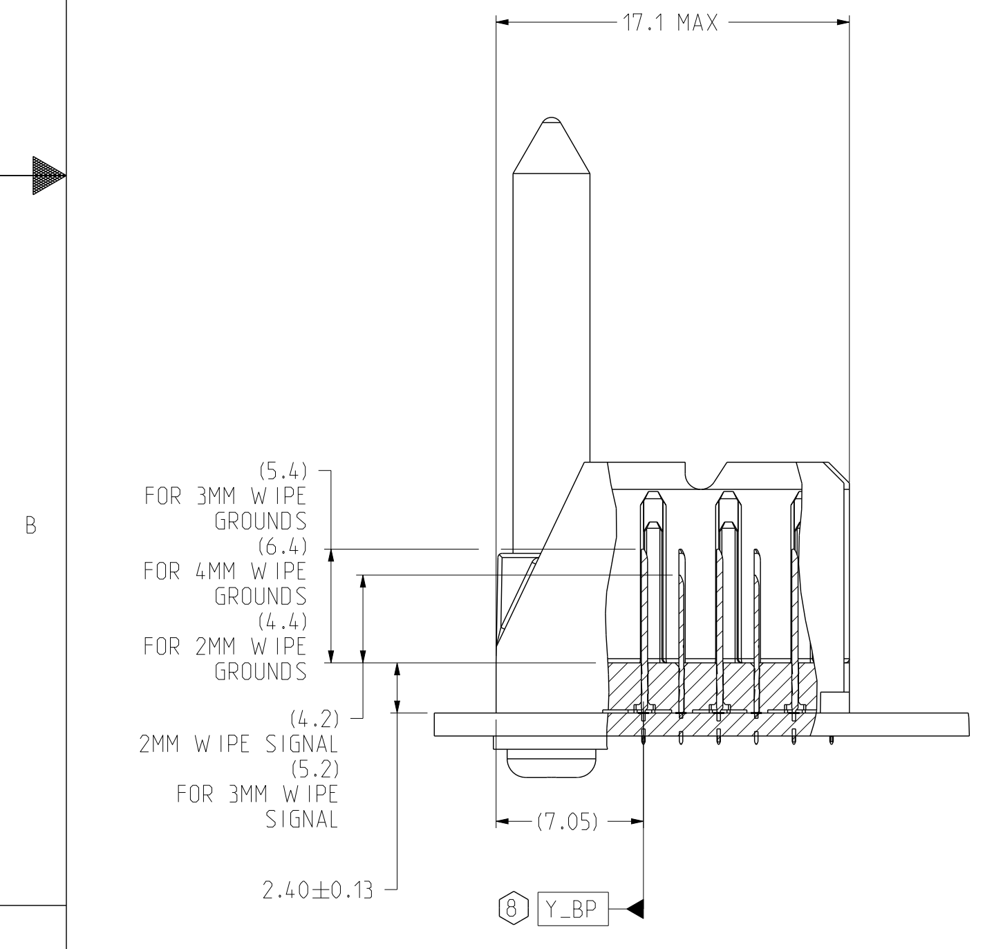
SECTION Z-Z
