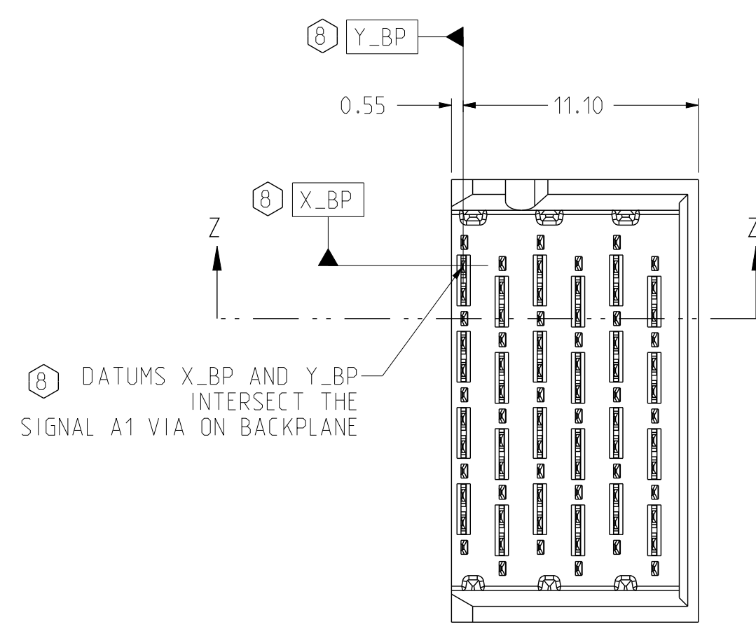
RIGHT WALL BACKPLANE MODULE DIMENSION
