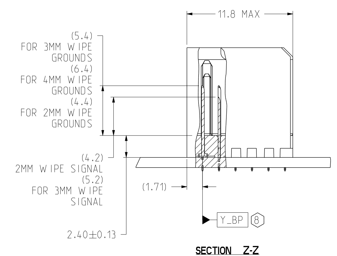
SECTION Z-Z
