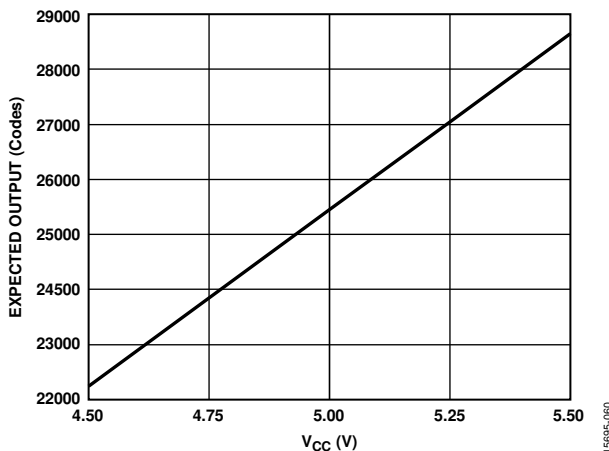
Figure 59. V CC Diagnostic Transfer Function
