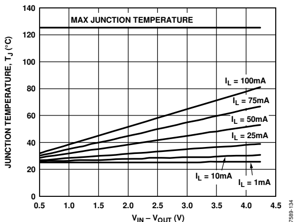
Figure 34. TSOT, 500 mm 2 of PCB Copper, T A = 25°C
