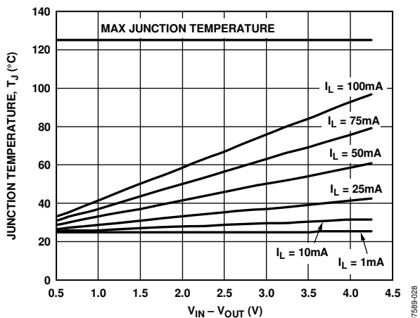
Figure 36. TSOT, 0 mm 2 of PCB Copper, T A = 25°C
