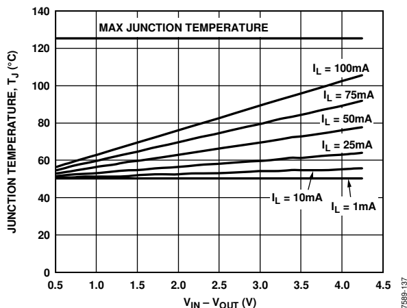
Figure 37. TSOT, 500 mm 2 of PCB Copper, T A = 50°C
