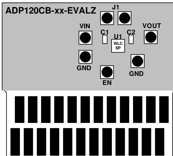
Figure 49. WLCSF PCB Layout
