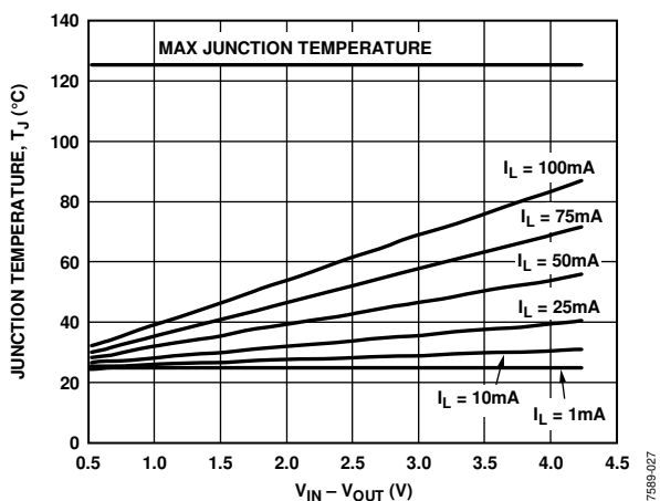
Figure 35. TSOT, 100 mm 2 of PCB Copper, T A = 25°C
