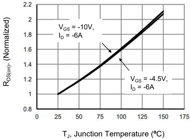
Figure 7. Drain-Source On-Resistance
