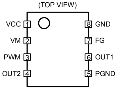
Figure 2. Pin Configuration
