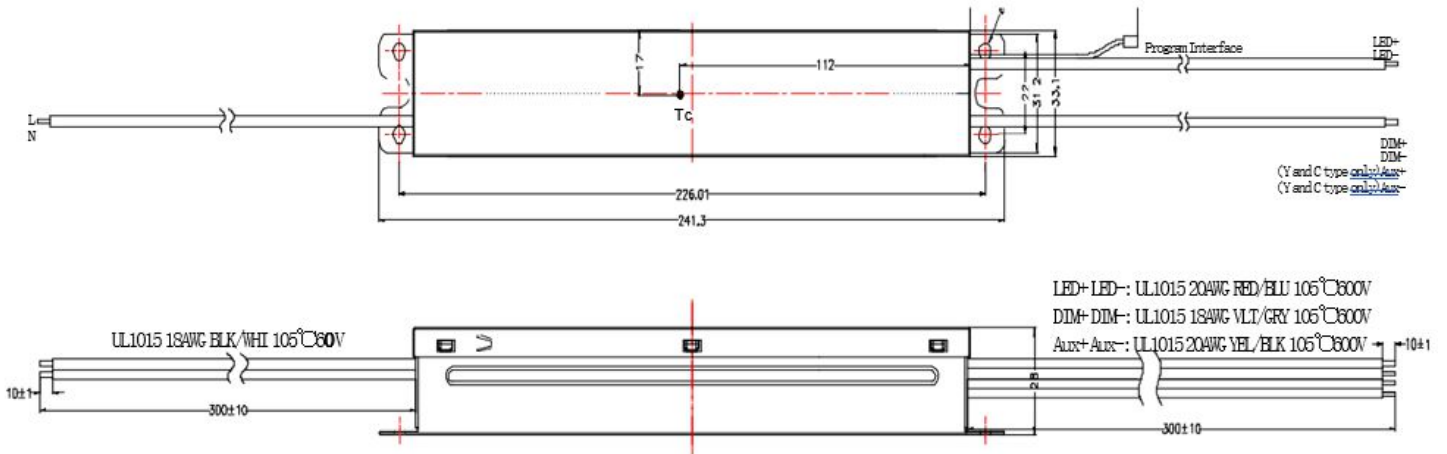
Figure 11: Mechanical Drawing
