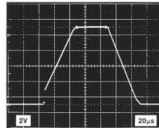
Figure 4. Large-Signal Transient Response ( A_{VCL} = 1 )
