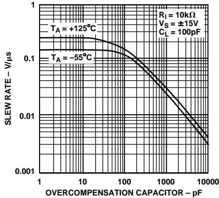
TPC 23. Slew Rate vs. Overcompensation
