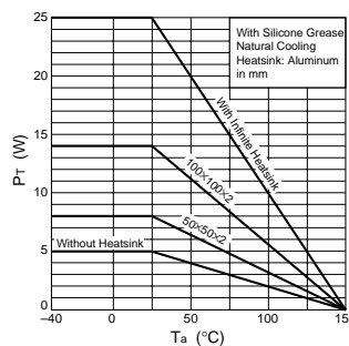
Pr-Ta Characteristics
