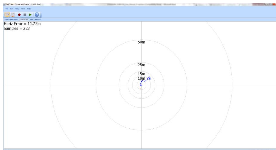
Figure 9 Scatter Plot
