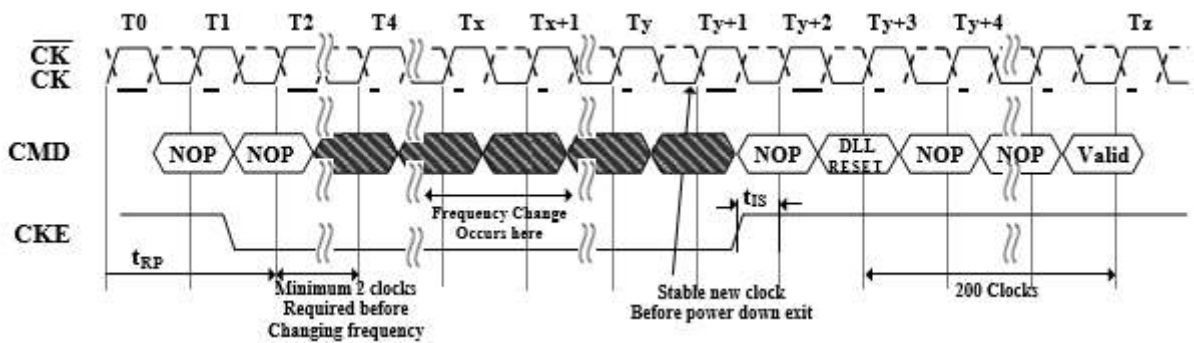
Figure 29. Clock Frequency Change in Precharge
