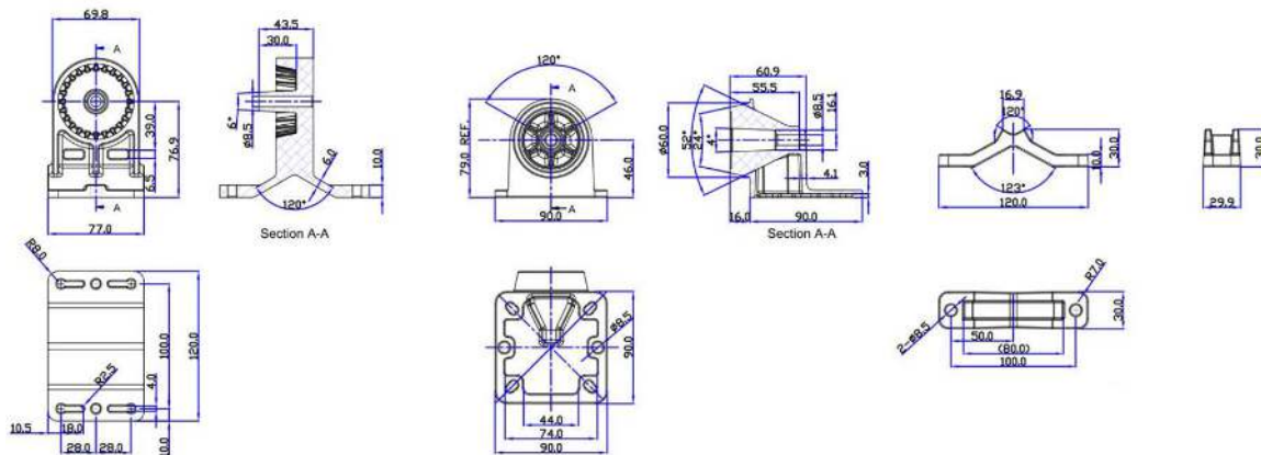
Figure 74: Pole mount dimensions
