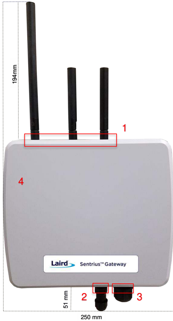
Figure 58: Top of the IP67 Rated Sentrius™ RG1xx Gateway
