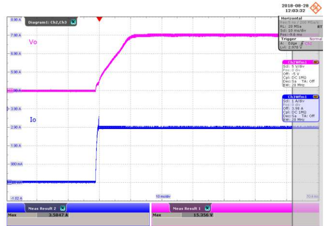
Figure 74 – Output Voltage and Current Waveforms. 135 VAC Input, 15 V, 5 Ω Load. Upper: V_{OUT} , 5 V / div Lower: I_{OUT} , 1 A, 10 ms / div.
