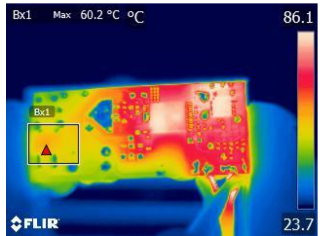
Figure 35 – Ambient = 23.7 °C. Bridge Diode, BR1 = 60.2 °C.
