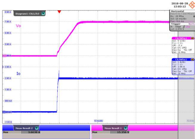
Figure 73 – Output Voltage and Current Waveforms. 100 VAC Input, 15 V, 5 Ω Load . Upper: V_{OUT} , 5 V / div Lower: I_{OUT} , 1 A, 10 ms / div.
