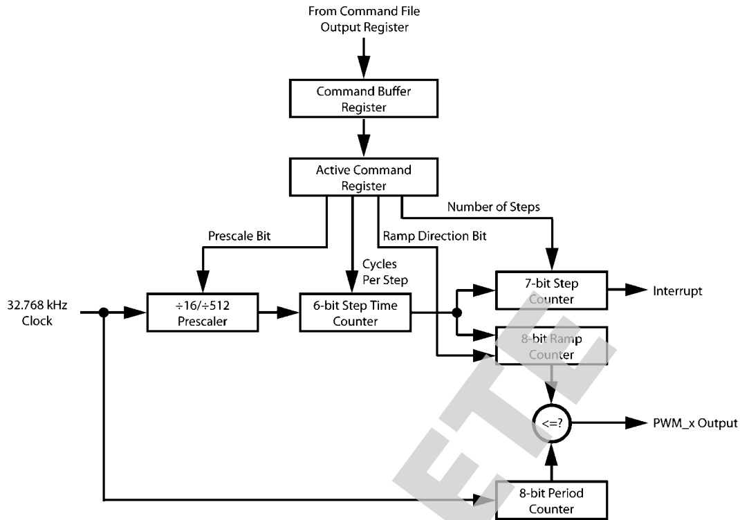
FIGURE 13. PWM Timer
