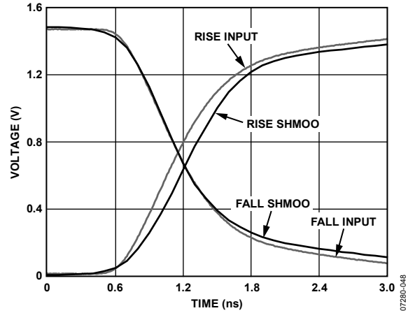
Figure 31. Comparator Shmoo, 1.5 V Input, 1.5 ns (10% to 90%) Input, 50 Ω Terminated
