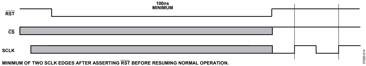
Figure 78. Reset Operation
