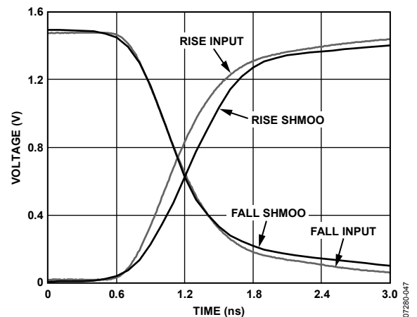
Figure 32. Comparator Shmoo, 1.5 V Input, 1.2 ns (10% to 90%) Input, 50 Ω Terminated
