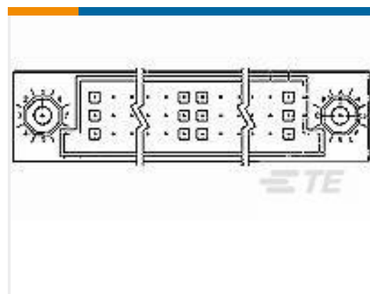
TE Part #532447-3 HDI PIN ASSY 3 ROW 96 POS
