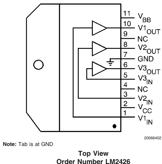
FIGURE 1. Simplified Connection and Pinout Diagram
