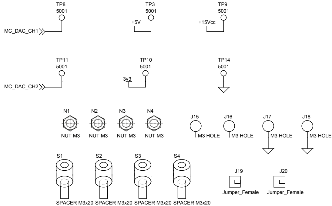
Figure 10. STEVAL-ETH001V1 circuit schematic (10 of 10)
