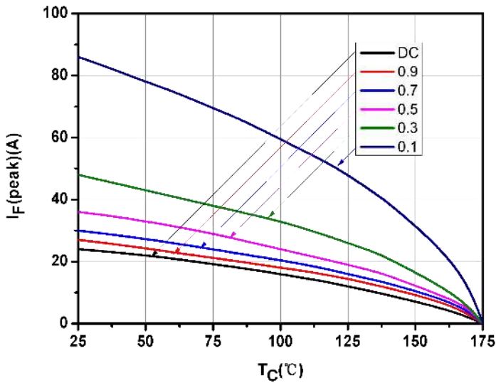
Fig.7-Current Derating
