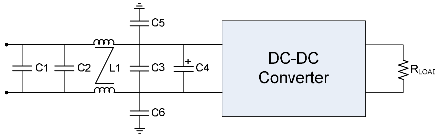
Figure 22. EMI Filter
