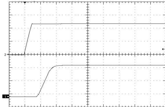
Figure 10. Startup Waveform via Input Voltage, time scale 10mS/div. Vin=Vin_nom, lout=full load Cout=1000uF, Ch1=Vout (5V/div), Ch2=Vin (20V/div)
