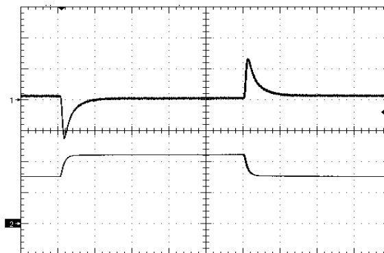
Figure 14. Transient Response (50mV/div), di/dt=0.1A/uS, 50%-75%-50% of full load, Cout=Fig3 time scale: 200uS/div. Ch1=Vout, Ch2=Iout (1A/div)
