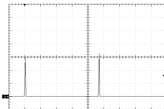
Figure 16. Short Circuit Current (2A/div), 10 milliohm short, time scale: 20mS/div Ch2=Iout
