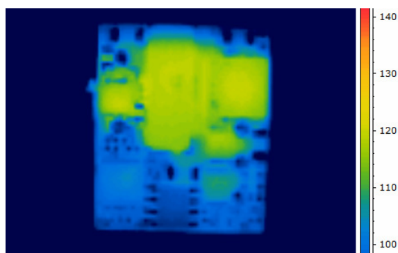
Figure 6. Thermal Image of CPZ3B48 3A output, 55C Ambient, 100lfm airflow, Vin = 48V, T_{max} = 123^{\circ}C
