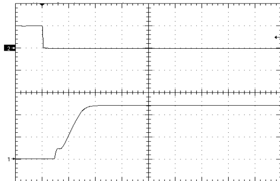
Figure 12. Startup Waveform via Enable Pin, time scale 10mS/div. Vin=Vin_nom, lout=no load Cout=0uF, Ch1=Vout (5V/div), Ch2=Enable (5V/div)
