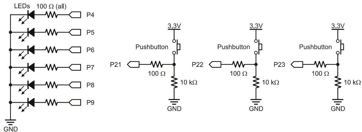
Figure 4-1: LED Pushbutton Schematic
