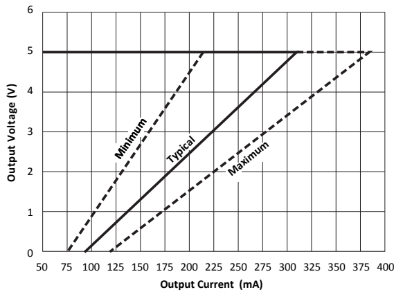
Figure 4. Foldback current limit of the 5V regulator
