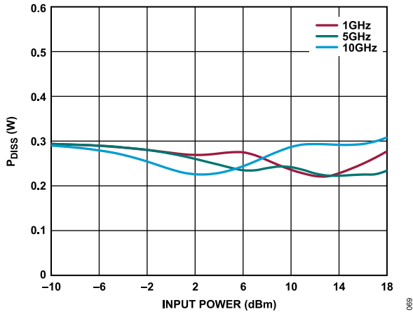
Figure 69. P_{DISS} vs. Input Power at T_A = 85^\circ\text{C} , V_{DD} = 5\text{ V} , I_{DQ} = 60\text{ mA}
