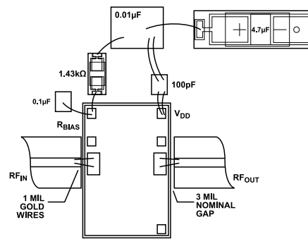
Figure 75. Assembly Diagram
