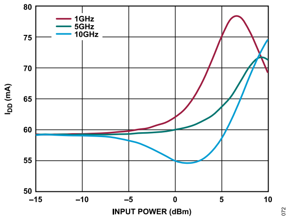
Figure 71. Drain Current ( I_{DD} ) vs. Input Power for Various Frequencies, V_{DD} = 5\text{ V} , R_{BIAS} = 1.43\text{ k}\Omega
