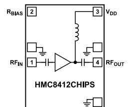
Figure 73. Simplified Block Diagram
