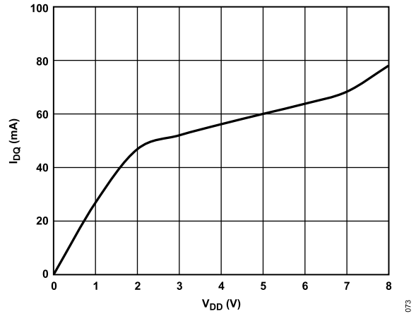
Figure 72. I_{DQ} vs. V_{DD} , R_{BIAS} = 1.43\text{ k}\Omega
