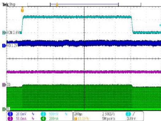
TPS62801 V_{OUT} = 1.2\text{ V} V_{IN} = 3.6\text{ V to } 4.2\text{ V} rise / fall time = 10\ \mu s I_{OUT} = 50\text{ mA}
