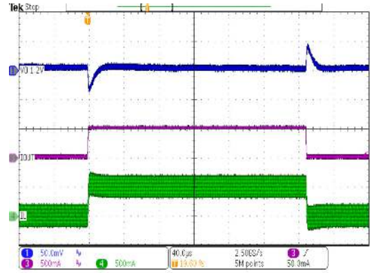
Forced V_{OUT} = 1.2\text{ V} VSEL/MODE = VIN PWM mode (after start-up) rise / fall time < 1\ \mu s I_{OUT} = 5\text{ mA to } 500\text{ mA}
