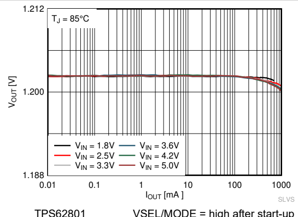
Figure 9-17. Output Voltage vs Output Current
