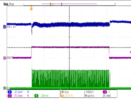
TPS62801 V_{OUT} = 1.2\text{ V} V_{SEL}/MODE = GND rise / fall time < 1 µs I_{OUT} = 0\text{ mA} to 50 mA, PFM Mode
