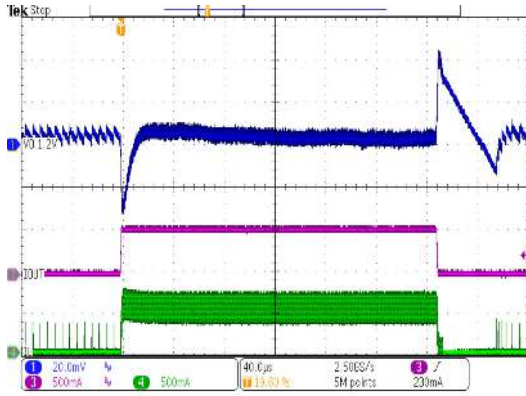
TPS62801 V_{OUT} = 1.2\text{ V} VSEL/MODE = GND rise / fall time < 1\ \mu s PFM / PWM mode I_{OUT} = 5\text{ mA to } 500\text{ mA}
