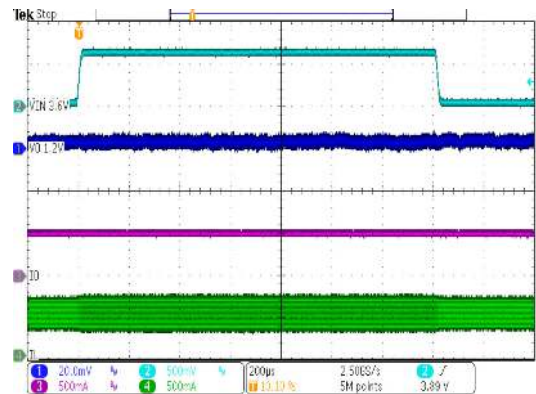
TPS62801 V_{OUT} = 1.2\text{ V} V_{IN} = 3.6\text{ V to } 4.2\text{ V} rise / fall time = 10\ \mu s I_{OUT} = 500\text{ mA}
