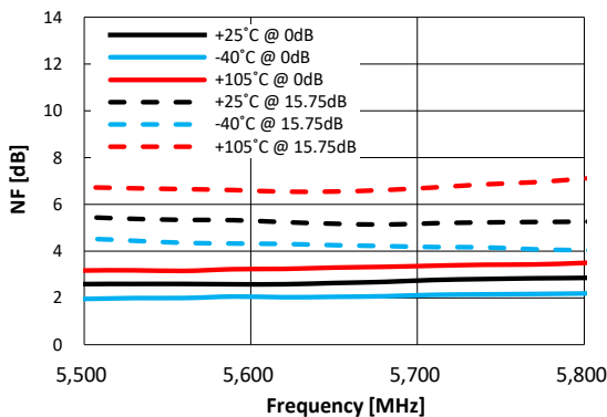
Figure 108. Noise Figure vs. Frequency @ VDD = 5V Over Temperature
