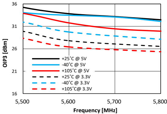
Figure 105. OIP3 vs. Frequency vs. VDD Over Temperature (Max Gain State)
