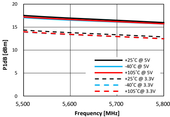
Figure 107. P1dB vs. Frequency vs. VDD Over Temperature (Max Gain State)
