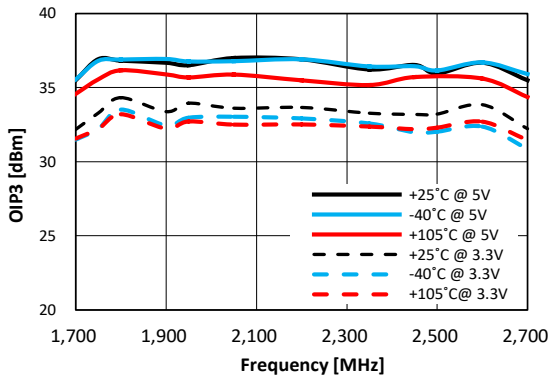
Figure 51. OIP3 vs. Frequency vs. VDD Over Temperature (Max Gain State)
